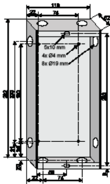
Flush mount back box
